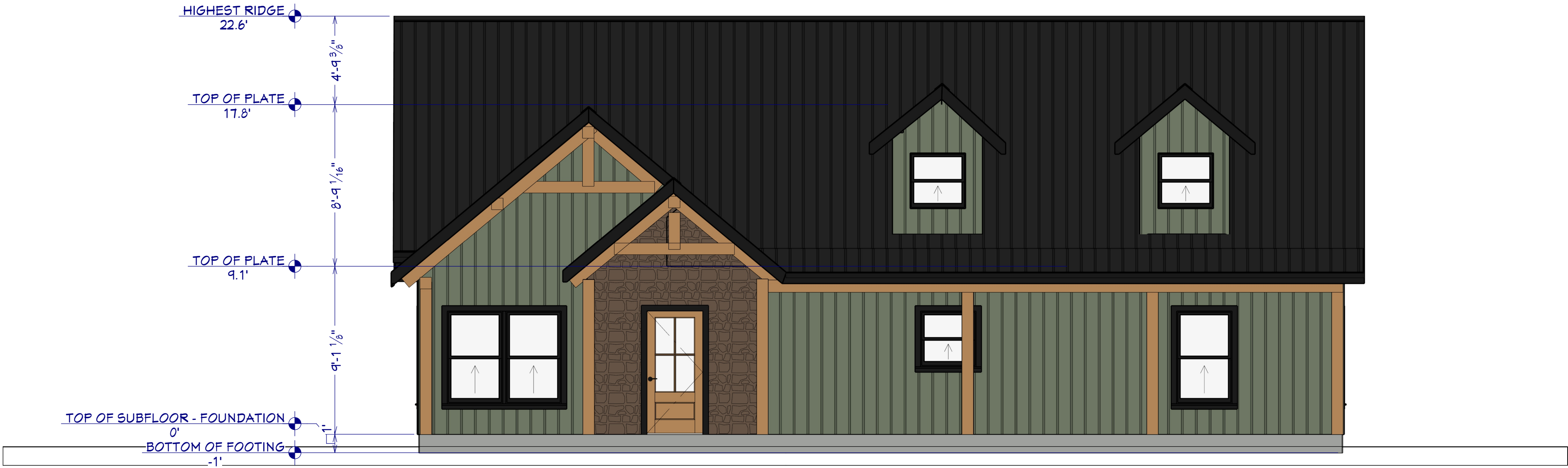
Exterior Elevation Front
